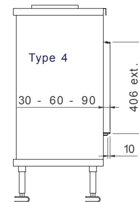
Luna Diamond 1300H Gas/Gaz
